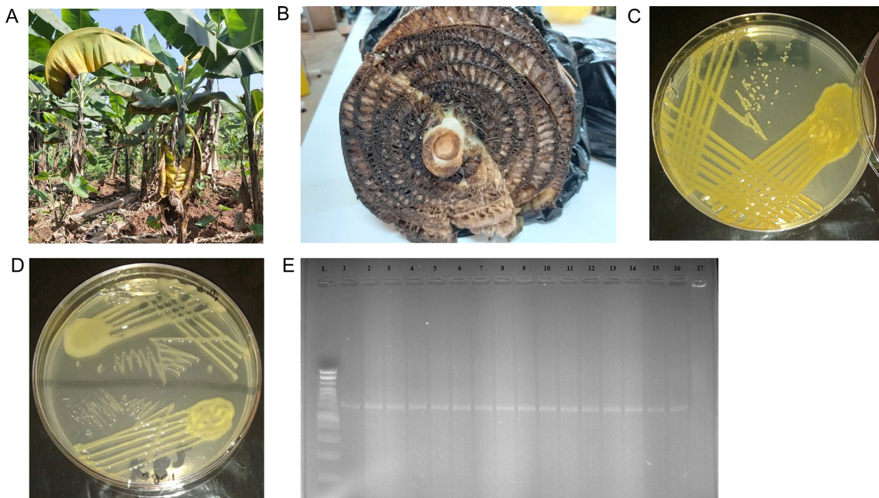
Fig. 1 BXW-infected banana plant, pseudostem and bacteria isolates on YPGA-CC plates. A. Yellowing and wilting of leaves as symptoms for BXW. B. Pseudostem with yellowish exudate. C. Bacteria isolates with small yellow colonies situated at the center of the agar plate. D. Bacteria isolate that appears as a yellowish mucoid colony after four days of incubation. E. Confirmation of Xvm by PCR. Lane L: 1000 bp ladder, Lane 1–17: Xvm 9-7, Xvm 1-4, BS17-5, BS17-6, BS8b2, Ooze 3b, L, P1, B6, AB14, B3 7, BCC280, U40L2, BCC 278, U09L3b, KB1, E3
