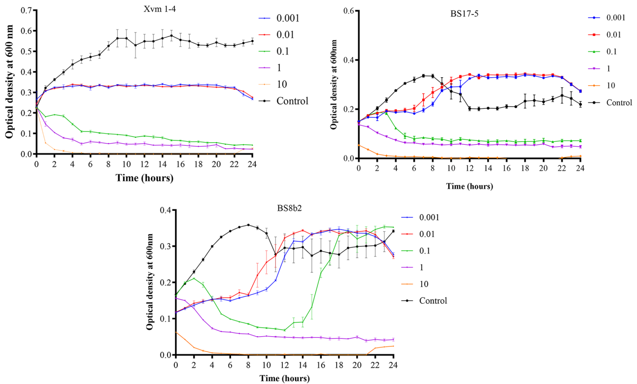
Fig. 5 Growth inhibition of Xvm 1-4, BS17-5, BS8b2 by Kintu at MOI 0.001, 0.01, 0.1, 1 and 10. The y-axis represents optical density (OD) at 600 nm, while x-axis represents time in hours. Error bars represent the mean \pm standard deviation from three independent experiments, each performed in triplicate
