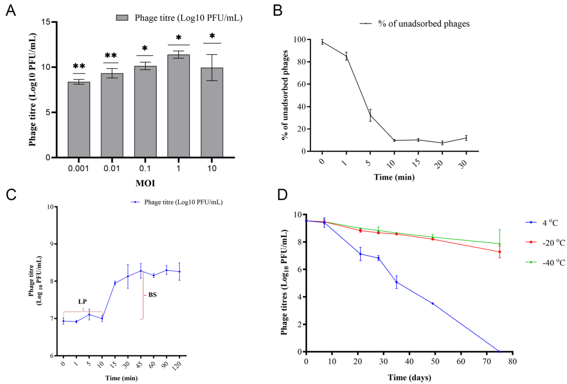
Fig. 3 Replication parameters and storage effects of Kintu phage at different temperatures. A. Shows MOI at ratios of 0.001, 0.01, 0.1, 1 and 10. ** indicates a statistically significant difference ( p < 0.05 ), while * indicates no statistically significant difference ( p > 0.05 ). Phage titers are expressed in PFU/mL. B. Percentage of unadsorbed phage over time. C. One-step growth curve showing a latent period (LP) of 10 min and a burst size (BS) of 15 PFU/cell. D. Phage stability at different storage temperatures (4 °C, -20 °C and -40 °C). Error bars represent the mean \pm standard deviation from three independent experiments, each performed in triplicate
