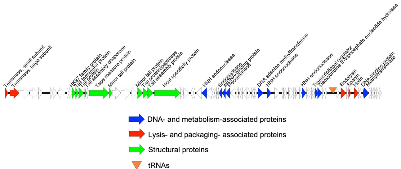
Fig. 6 Genome map of Kintu. Each arrow represents a coding sequence on the Kintu genome. The coding sequences were colored according to the function of the encoded protein: blue represents proteins associated with DNA replication and general metabolism; red represents proteins associated with lysis and packaging; green represents structural proteins; and white represents hypothetical proteins. Two tRNA genes were retrieved on the Kintu genome, displayed as an orange triangle
