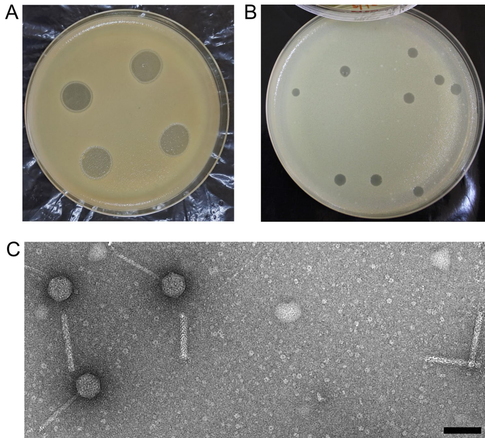
Fig. 2 Phage detection and phenotypic characterization. A. Zone of lysis by sewage filtrate on an Xvm9-7 lawn. B. Circular and clear plaques with a diameter of 3 mm on YPG agar plates. C. Transmission electron micrograph of Kintu displaying a siphovirus morphology. Scale bar represents 100 nm
